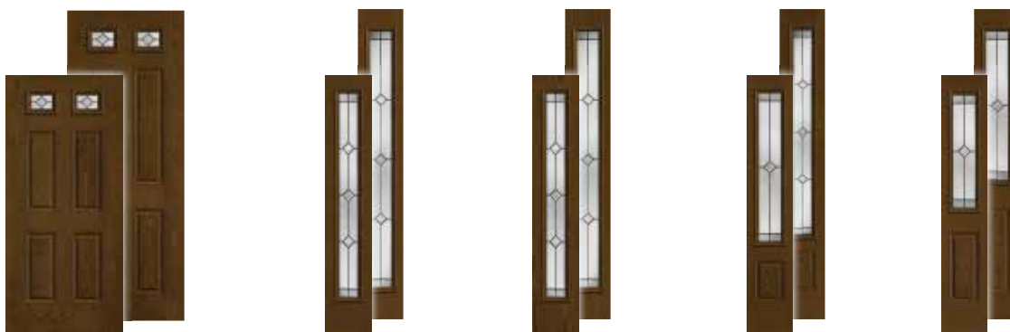
FC6570 9 2'6" x 6'8" ‡ 2'8" x 6'8" 2'10" x 6'8" 3'0" x 6'8" FC86570 9 2'8" x 8'0" 3'0" x 8'0" FC6550SL 9 10" x 6'8" 12" x 6'8" 14" x 6'8" FC86550SL 9 12" x 8'0" 14" x 8'0" FC6500SL 9 12" x 6'8" † ‡ 14" x 6'8" † ‡ FC86500SL 9 12" x 8'0" 14" x 8'0" FC6580SL 9 12" x 6'8" 14" x 6'8" FC86580SL 9 12" x 8'0" 14" x 8'0" FC6565SL 9 12" x 6'8" 14" x 6'8" FC86560SL 9 12" x 8'0" 14" x 8'0"
